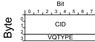
Figure 13: Vendor Specific Query message
